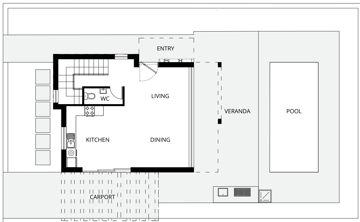
GROUND FLOOR
